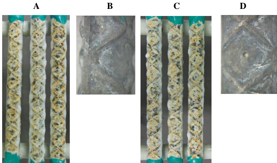
Figure 4. Appearance of Type A galvanized bars after 174 hours of exposure. A) no hole; B) no hole after cleaning; C) with a hole; D) with a hole after cleaning
